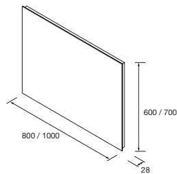
Espejo BLOCK 1000 horizontal vertical luz led (25 W-5700°K) IP44 - 700 x 1000 mm 105598
