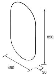
Espejo Thais vertical con luz led (12 W - 5700°K) IP 44 450 x 850 mm 105599
